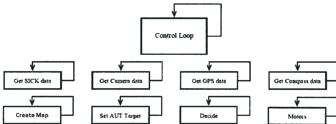
Figure 5: Parallel architecture used for IGVC 2011. Here, each block represents a process running in a loop in separate LabVIEW VIs.
