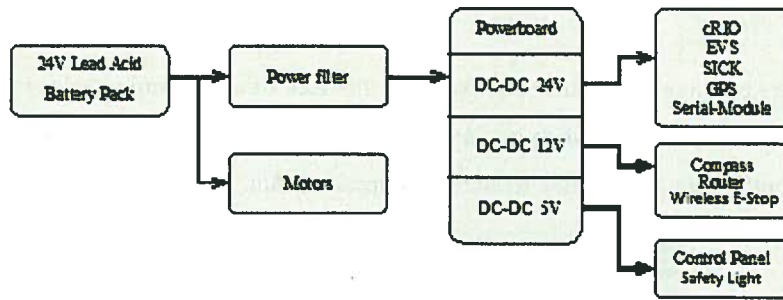
Figure 5: Power Distribution and Electrical System
