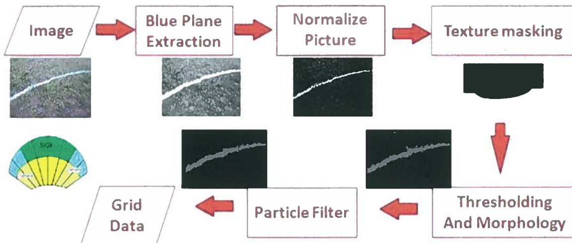
Figure 11: Image Processing Loop
